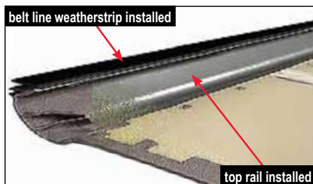
pre-assembled door panel - sample photo includes upper rail and belt line weatherstrip
